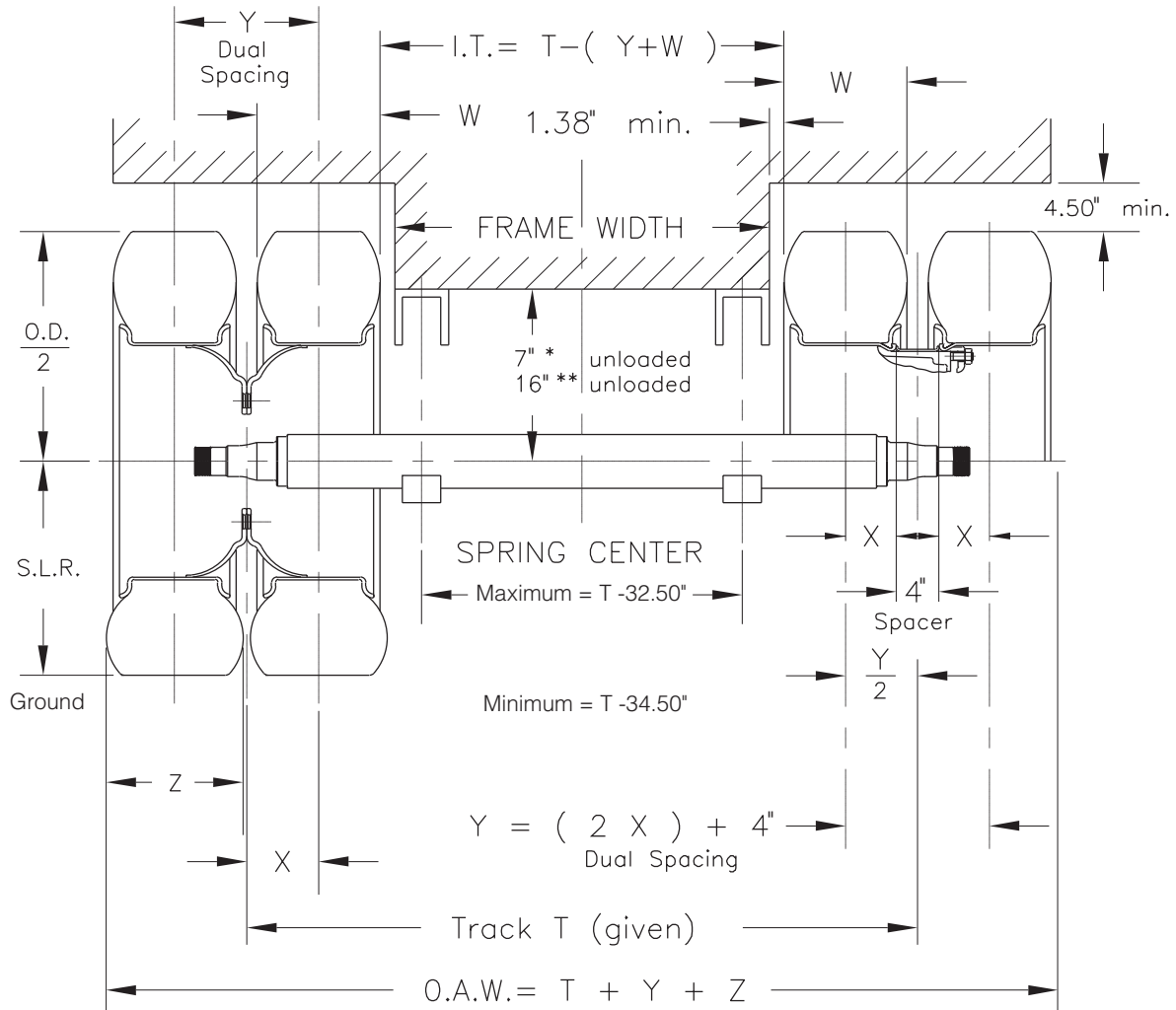
Disc Wheel
